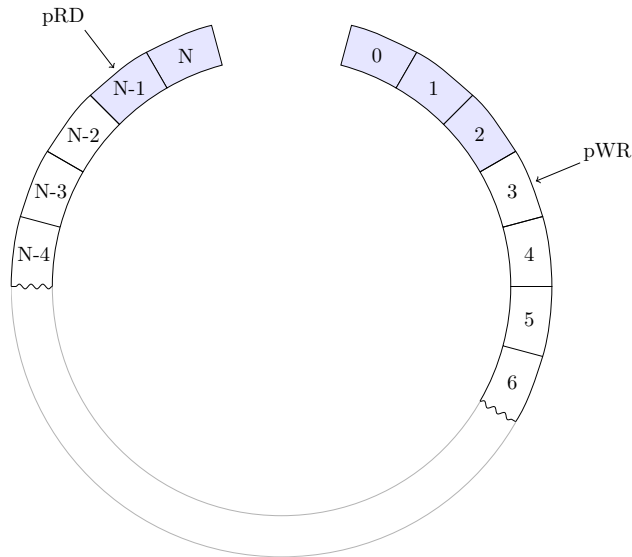
Figure 11.5: Circular Buffer
